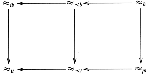
FIGURE 8. Some semantic equivalences on \mathbb{E}(\text{Act}^\pm)
