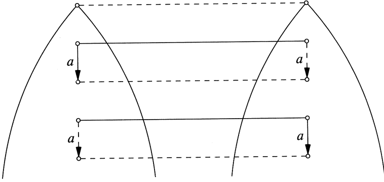
FIGURE 8. A bisimulation
